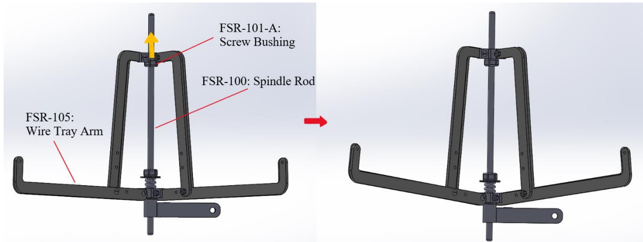
Figure 6 Screw bushing is slid up the spindle rod to raise the wire tray arms, or slid down to lower the arms.
